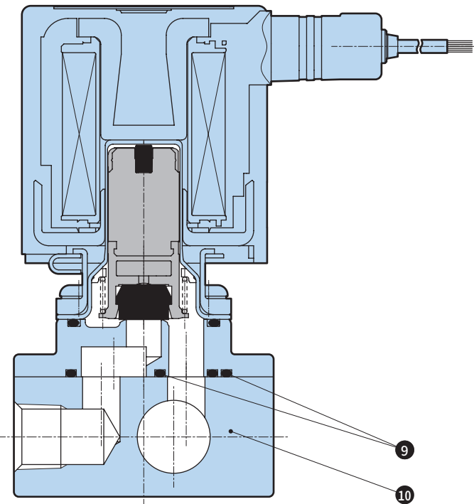
● FFBM 集成阀
